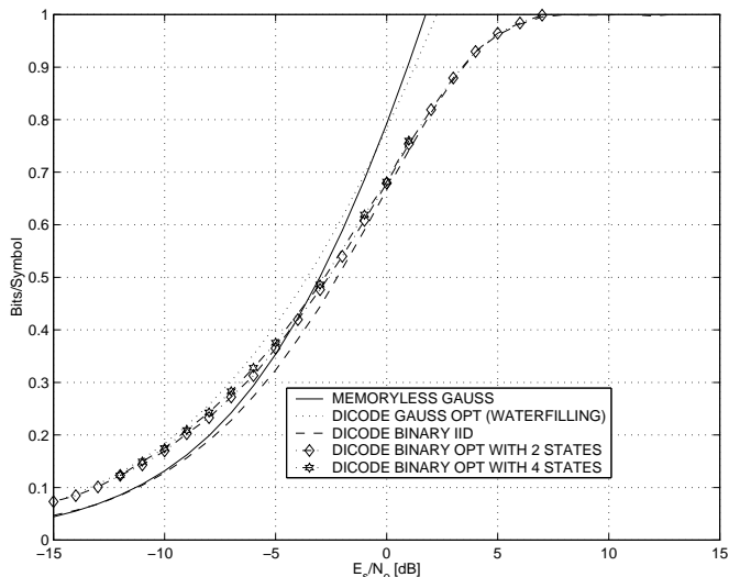
Fig. 5. Maximum information rates of the DICODE channel for input processes with memory 0, 1, and 2.
