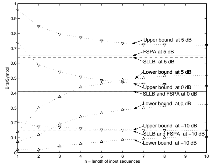
Fig. 4. Comparison of uniform-input information rates obtained by different methods for the CH6-channel.
