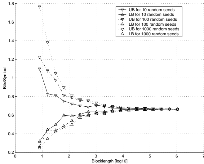
Fig. 2. Convergence behaviour of the new algorithm.
