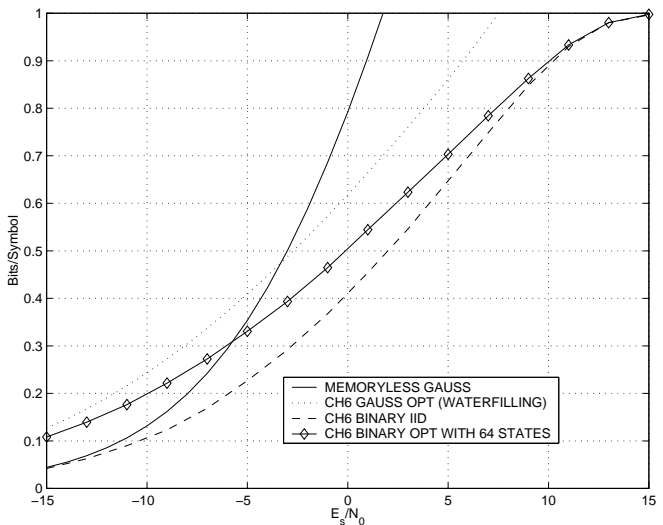
Fig. 6. Maximum information rate of the CH6 channel for an input process with memory 6.
