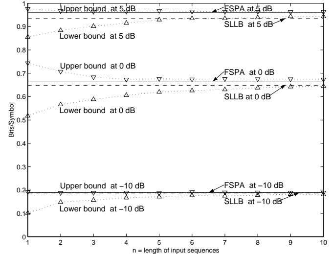
Fig. 3. Comparison of uniform-input information rates obtained by different methods for the DICODE-channel.
