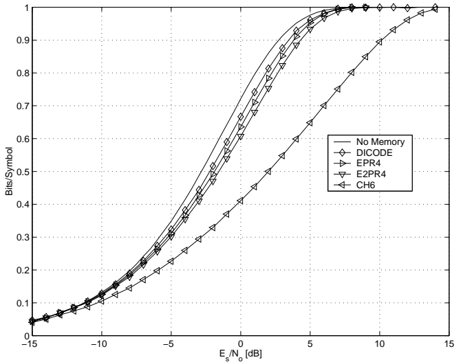
Fig. 1. Uniform-input information rates of selected channels.
