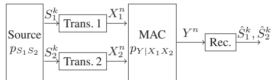
Fig. 1: MAC without feedback
