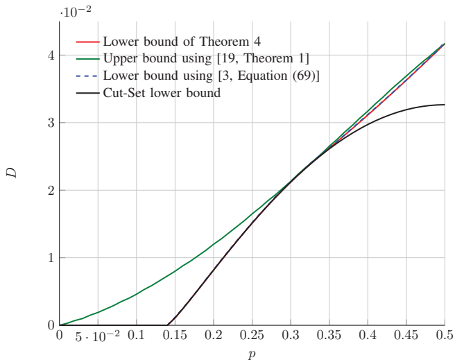
Fig. 3: Distortion upper and lower bounds as functions of p .
