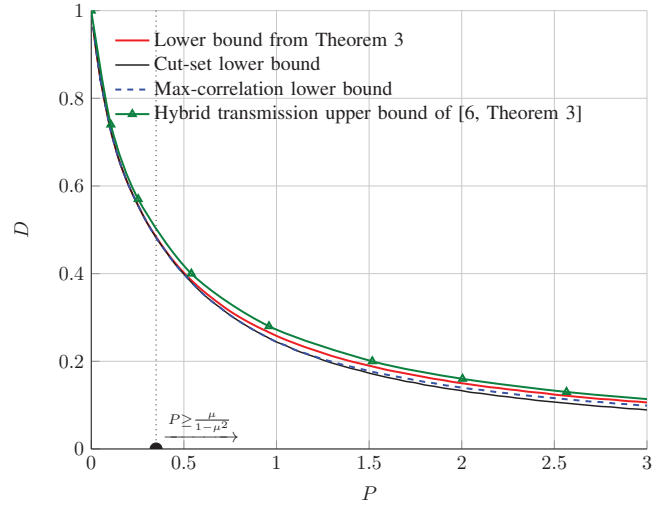
Fig. 2: Bounds on the minimum achievable distortion D as a function of P for \sigma^2 = 1 , \rho = 0.4 , and \kappa = 0.5 .
